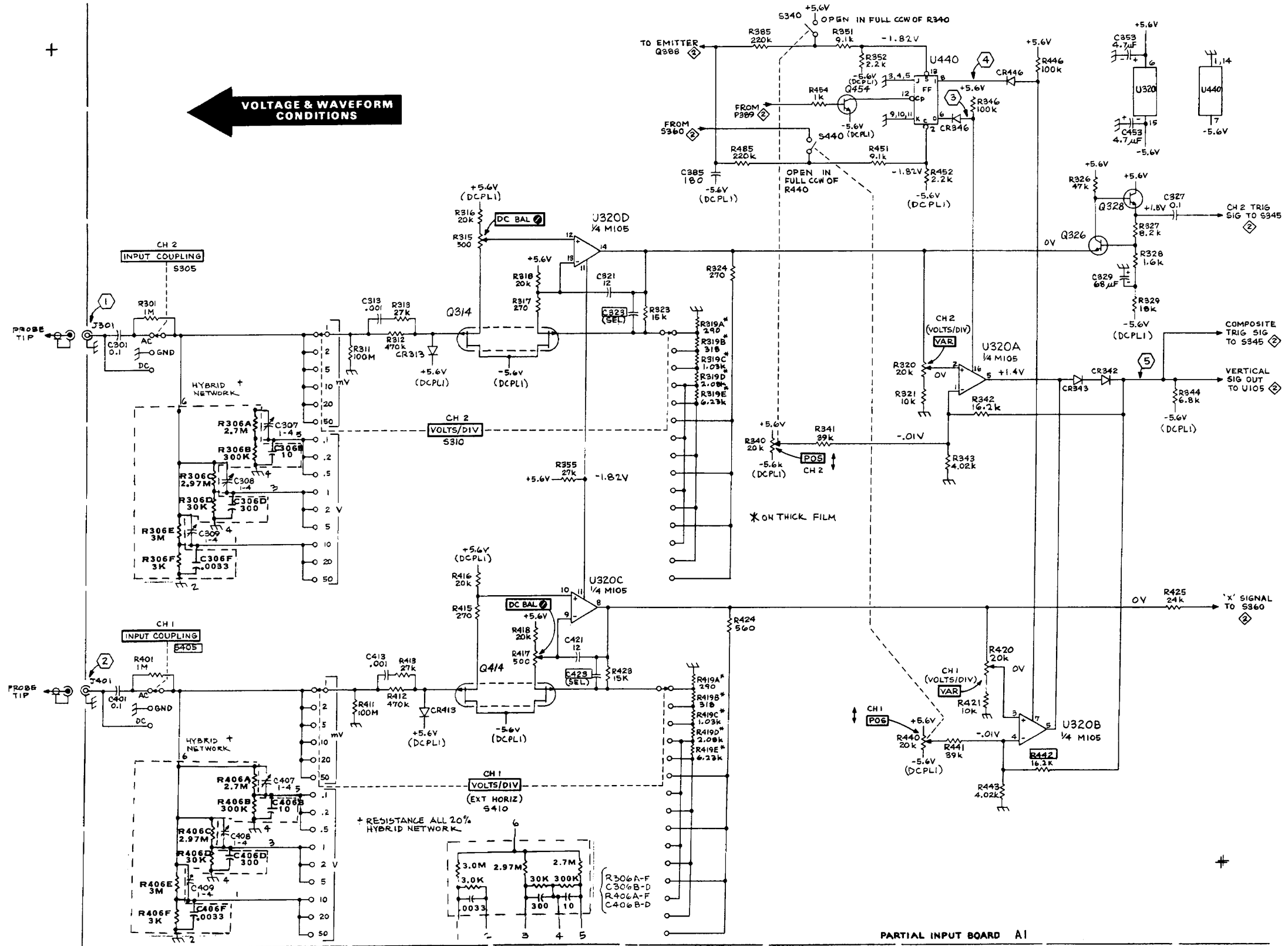
Figure 8-1D. Vertical Amplifier
